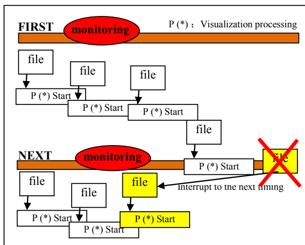
Fig. 9. Practice image of the parallelization
